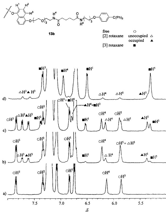
Figure 9. Partial ^1\text{H} NMR (500 MHz) spectra of a mixture of 2 + 13b in \text{CDCl}_3 at 10 °C: a) 13b (2 mM), b) 13b (2 mM) and 2 (1 mM), c) 13b (2 mM) and 2 (2 mM), and d) 13b (2 mM) and 2 (4 mM).
