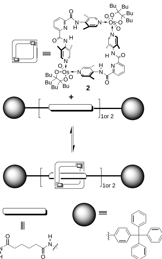
Figure 1. Schematic representation for the reversible formation of rotaxanes studied here.
