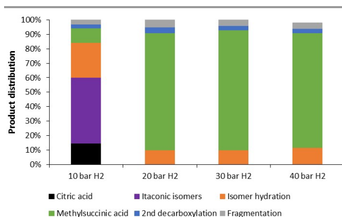
Figure 6. Effect of H 2 pressure on the conversion of citric acid to methylsuccinic acid using the carbon-coated Ni nanoparticles. Reaction conditions: citric acid (0.2 mmol), Ni-C NPs (10 mol% Ni), water (2 mL), 175°C, 2 bar N 2 , 6 h.
