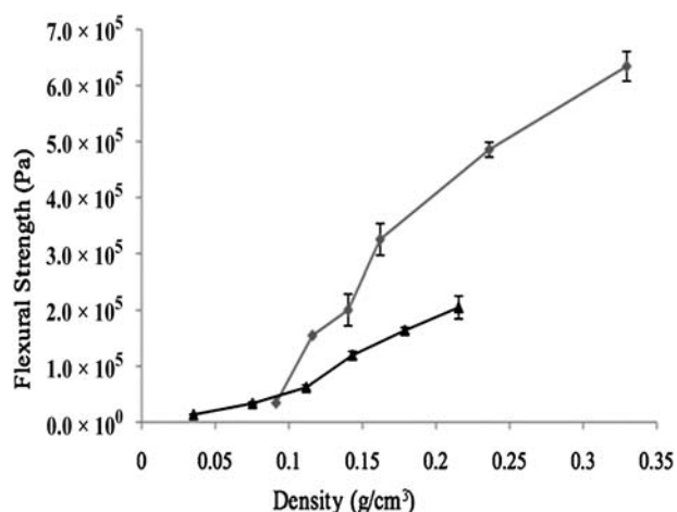
Fig. 3 Flexural strength as a function of density for PMMA-silica aerogel composites. The triangle line is for polymer free silica aerogels, and diamond line is for PMMA-silica aerogel composites.
