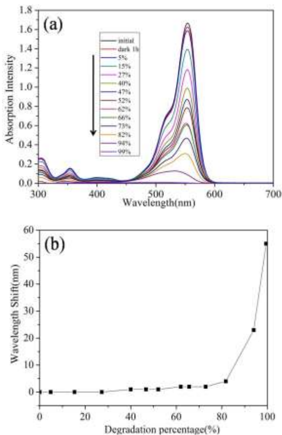
Figure 4 (a) UV-Vis absorption spectra of RhB dye solutions with different degradation percentage in Ag-BTO system and (b) The maximum absorption wavelength shift of RhB as a function of degradation percentage in Ag-BTO system
