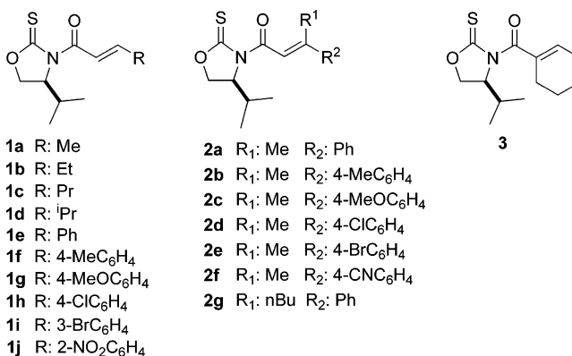
Scheme 1. General Pictogram of the Intramolecular Sulfur Transfer in N -Enoyl Cyclic Thiocarbamates (Oxazolidine-2-thiones) Promoted by Lewis Acids
