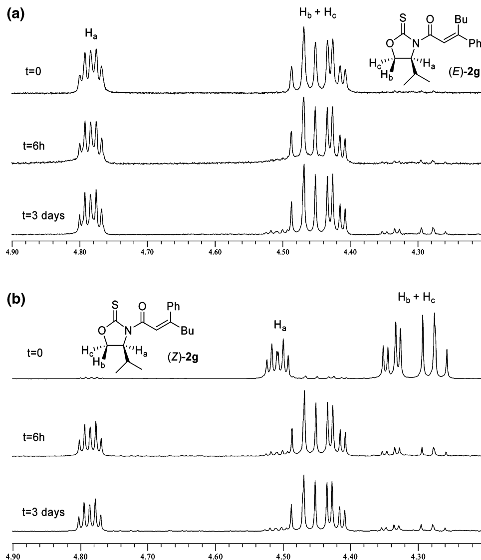
Figure 1. ^1\text{H} NMR plot inserts (4.20–4.90 ppm) corresponding to starting compound 2g and aliquots taken at 6 h and 3 days from a solution of 2g , \text{BF}_3\text{OEt}_2 (2 mol equiv), and 2,6-di- tert -butylpyridine (2.5 mol equiv) in \text{CH}_2\text{Cl}_2 at -30^\circ\text{C} : (a) starting from E - 2g ; (b) starting from Z - 2g .
