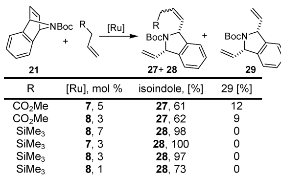
Scheme 5. ROCM of Boc-Protected 7-Azabicycloalkene 21
