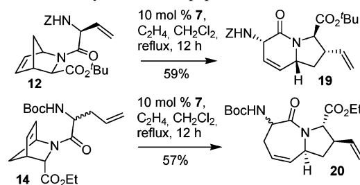
Scheme 3. Synthesis of Dipeptide Mimetics 19 and 20
