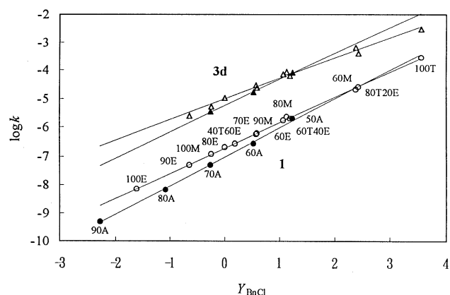
Figure 1. Correlations of \log k for (○) 1 and (Δ) 3d vs Y_{\text{BnCl}}
