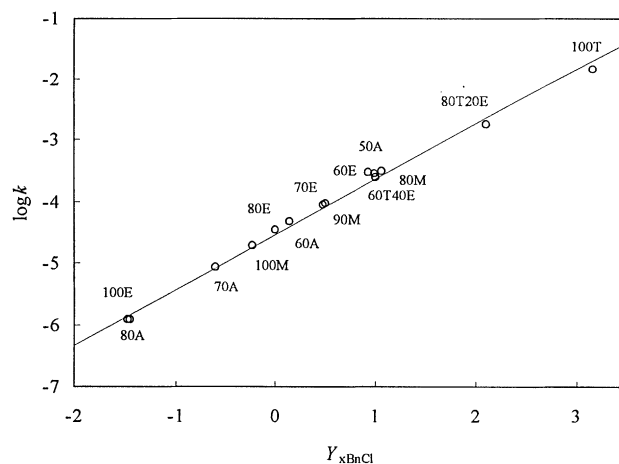
Figure 2. Correlations of \log k for (O) 3c vs Y_{\text{xBnCl}}
