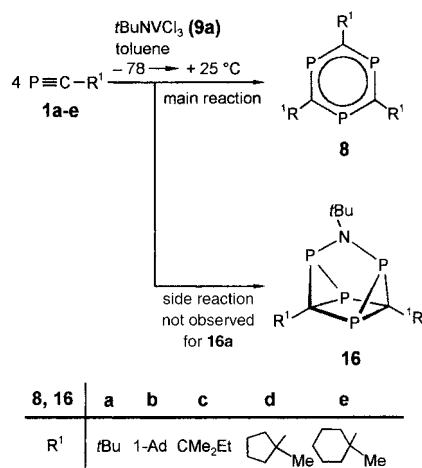
Scheme 6. Synthesis of 1,3,5-triphosphabenzene 8 .
