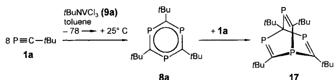
Scheme 7. Catalytic cyclotrimerization of 1a .
