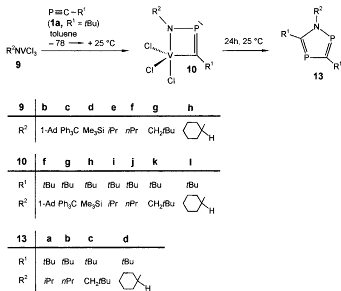
Scheme 4. Stable and unstable complexes 10 , synthesis of 1 H -1,2,4-azadiphospholes 13 .
