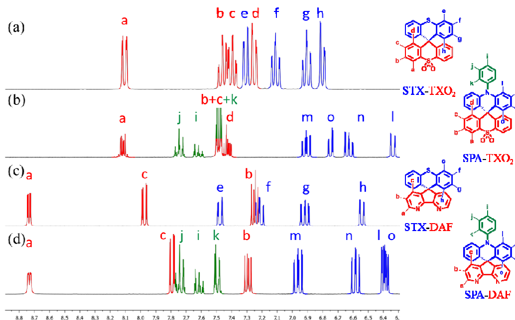
Figure 1. Portion 1 H of NMR Spectra of (a) STX-TXO 2 , (b) SPA-TXO 2 , (c) STX-DAF and (d) SPA-DAF in CD 2 Cl 2 .
