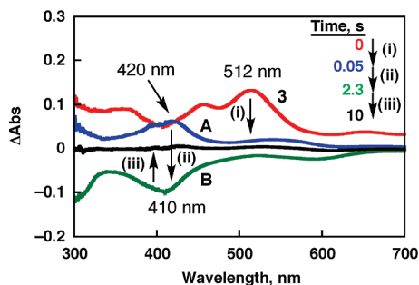
Figure 2. UV-vis difference absorption spectral changes observed in the reduction of \text{O}_2 (0.13 mM) by 3 (red line, 0.10 mM) in the presence of \text{HCOOH}/\text{HCOONa} (0.10 M) in \text{H}_2\text{O} at pH 5.2 at 298 K.
