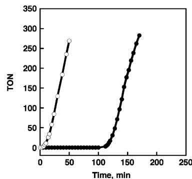
Figure 3. Time course of the turnover number (TON) of the \text{H}_2 evolution in the decomposition of \text{HCOOH}/\text{HCOONa} (0.83 M) catalyzed by 1 (0.5 mM) in deaerated (freeze–pump–thaw cycles, 5 times) \text{H}_2\text{O} (○) and in aerated \text{H}_2\text{O} (●) at pH 3.6 at 298 K.
