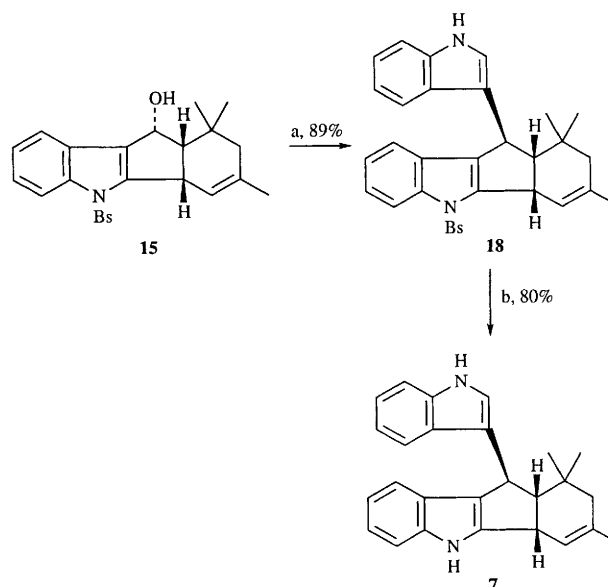
Scheme 4 Reagents and conditions: a, indole, \text{BF}_3 \cdot \text{Et}_2\text{O} , \text{Et}_2\text{O} , 0^\circ\text{C} ; b, \text{Na/Hg} , \text{Na}_2\text{HPO}_4 , \text{Et}_2\text{O-MeOH} , rt
