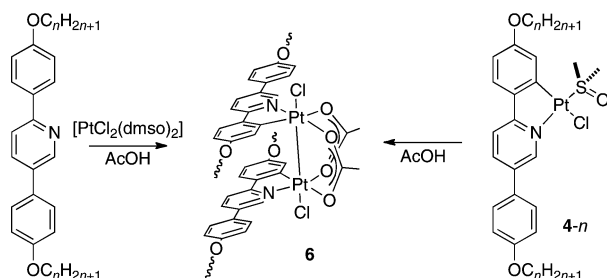
Chart 2. Molecular Structure of 6-2,1 a
