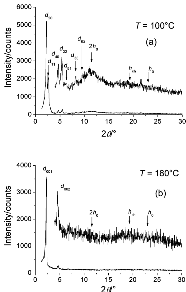
Chart 3. Small-Angle X-ray Diffraction Pattern for 6-14,1 at 100 °C (a) and 180 °C (b)
