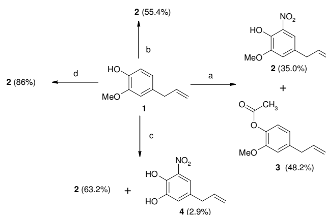
Scheme-I: Synthesis methods of nitro-eugenol ( 2 ). Conditions: (a) \text{HNO}_3/\text{CH}_3\text{COOH} , rt, 1 h, refluxed 20 min, (b) \text{HNO}_3/\text{dilute H}_2\text{SO}_4 , heated 55 °C, 20 min, (c) \text{NaNO}_3/\text{KHSO}_4\text{SiO}_2/\text{H}_2\text{O} (1:1) \text{CH}_2\text{Cl}_2 rt, 5.5 h, (d) \text{NH}_4\text{NO}_3/\text{KHSO}_4 , \text{CH}_3\text{CN} , rt, 0.5 h, refluxed 5 h
