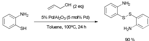
Figure 5 2-aminothiophenol formed the corresponding disulphide instead of the benzothiazole derivative under the reaction conditions.
