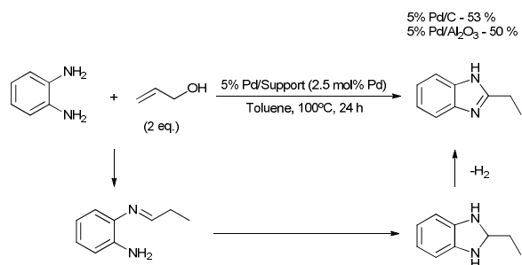
Figure 4 Supported Pd-catalysed one-pot isomerisation/imine formation/ring closing/dehydrogenation cascade reaction of allyl alcohol with o -phenylenediamine.
