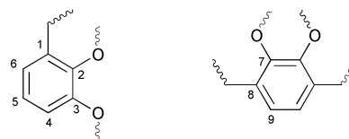
Scheme 8 Numbering of aromatic carbon atoms in catechol derivatives.
