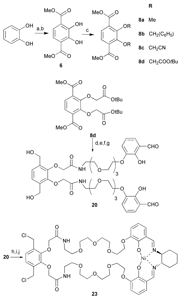
Scheme 6 Assembly of the protected catechol and convergence to the macrocycle 23 : a) 1) NaOH, MeOH, rt; 2) 110 °C, 3 days; 3) CO 2 , 70 bar, 200 °C, 2 days, 40% ( 5 ); b) MeOH, H 2 SO 4 , reflux, 8 h, 65% ( 6 ); c) K 2 CO 3 , MeCN, RX, reflux, 18–48 h, 70–95% ( 8a–d ); d) CF 3 COOH, rt, 3 h, 100% ( 17 ); e) 1) SOCl 2 , reflux, 1 h; 2) ( 16 ), Et 3 N, DMAP, CH 2 Cl 2 , 0 °C–rt, 74% ( 18 ); f) 1) LiAlH 4 , THF, 0 °C to rt, 2 h; 2) H + , 99% ( 19 ); g) Pd(OAc) 2 , P(C 6 H 5 ) 3 , Et 3 N, HCOOH, EtOH–H 2 O, reflux, 1.5 h, 62% ( 20 ); h) (±)- trans -cyclohexane-1,2-diamine, Ba(OTf) 2 , THF, reflux, 50% ( 21 ); i) Ni(OAc) 2 , MeOH, 1 min, 95% ( 22 ); j) MsCl, Et 3 N, CHCl 3 , 55 °C, 6 h, 95% ( 23 ).
