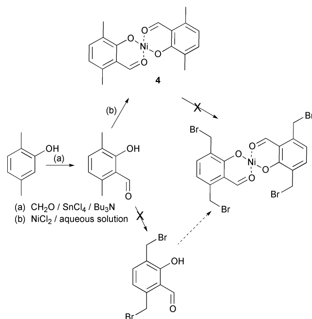
Scheme 3 Synthesis of the bis(dimethylsalicylaldehydato)nickel(II) dihydrate mediator 4 .
