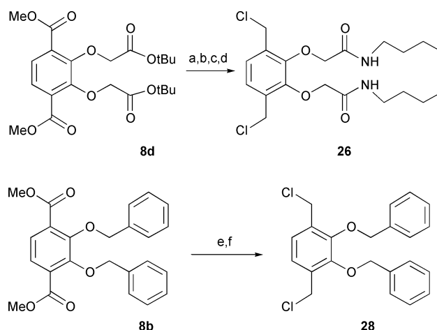
Scheme 7 Preparation of model compound 26 and 28 : a) CF 3 COOH, rt, 3 h, 100% ( 17 ); b) 1) SOCl 2 , reflux, 1 h; 2) n -BuNH 2 , Et 3 N, DMAP, CH 2 Cl 2 , 0 °C–rt, 84% ( 24 ); c) 1) LiAlH 4 , THF, 0 °C to rt, 2 h ( 25 ); 2) H + , 71%; d) SOCl 2 , 2,6-lutidine, rt, 1 h, quantitative ( 26 ); e) 1) LiAlH 4 , THF, 0 °C to rt, 2 h; 2) H + , quantitative ( 27 ); f) SOCl 2 , CH 2 Cl 2 , reflux, 1 h, quantitative ( 28 ).
