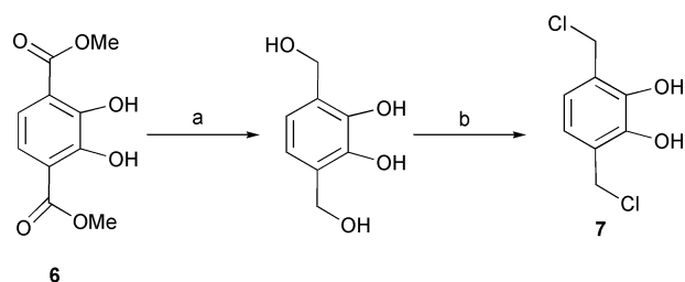
Scheme 4 (see also Scheme 6). Route to model compound 7 .
