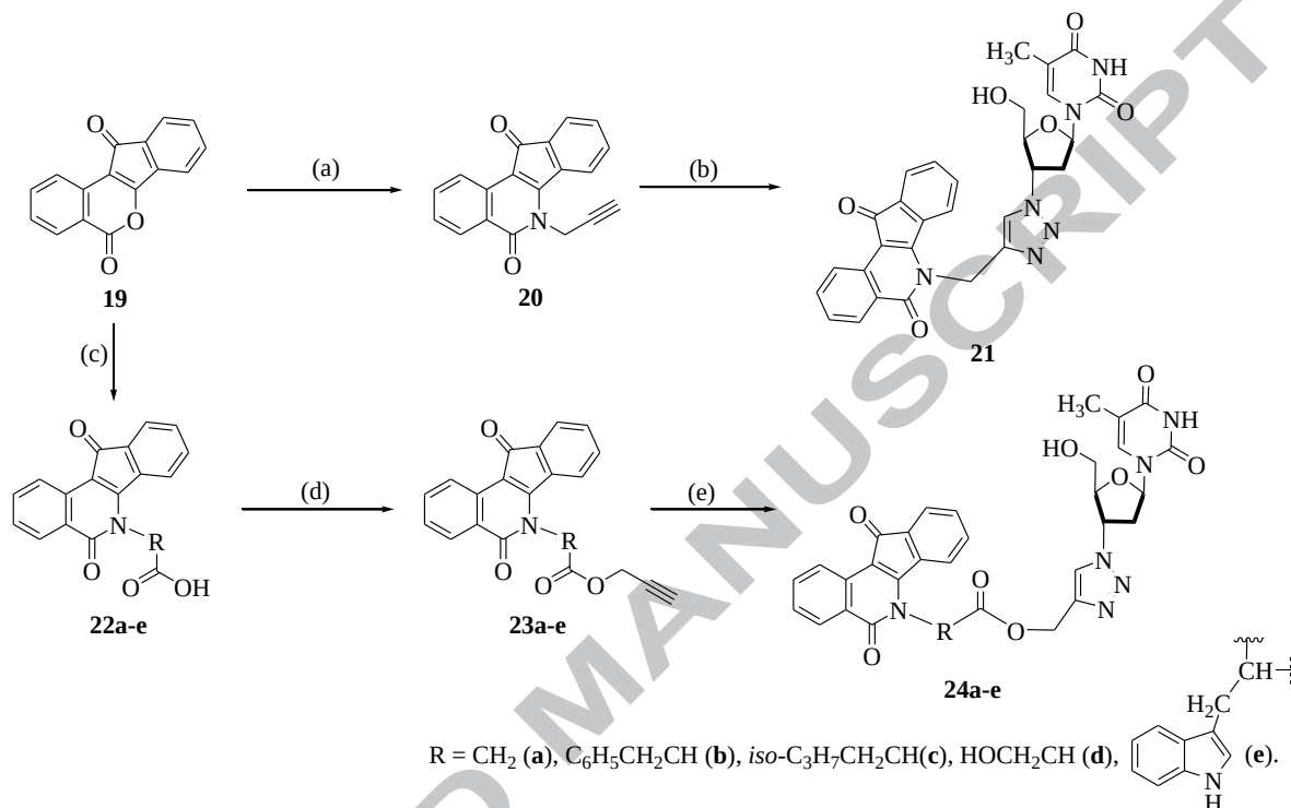
Scheme 2: Synthesis of triazole-indenoisoquinoline-AZT hybrids 21 and 24a-e . Reagents and conditions: (a) 1.1 equiv propargyl amine, CH 2 Cl 2 , 40°C, 24 h; (b) 0.9 equiv AZT, 0.2 equiv CuI, tert -BuOH, 70°C, 24 h; (c) 1.1 equiv amino acid, CH 2 Cl 2 , 40°C, 2-8 h; (d) 1.1 equiv propargyl bromide, 1.1 equiv Cs 2 CO 3 , DMF:THF (1:1), rt, 2-6 h; (e) 0.8 equiv AZT, 0.2 equiv DIPEA, 0.1 equiv CuI, THF, reflux, 24 h.
