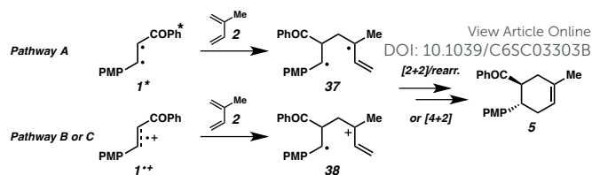
Fig. 4. General regiochemical explanation.
