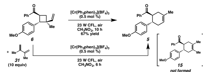
Scheme 3. Rearrangement of vinylcyclobutane 6 .
