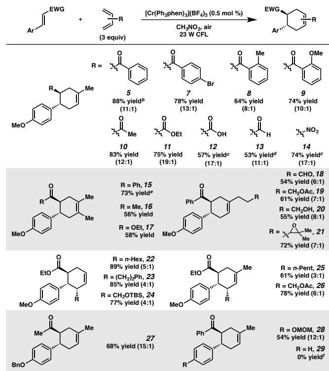
Scheme 2. The Cr-photocatalyzed [4+2] cycloaddition between dienes and electron-deficient alkenes - scope.
