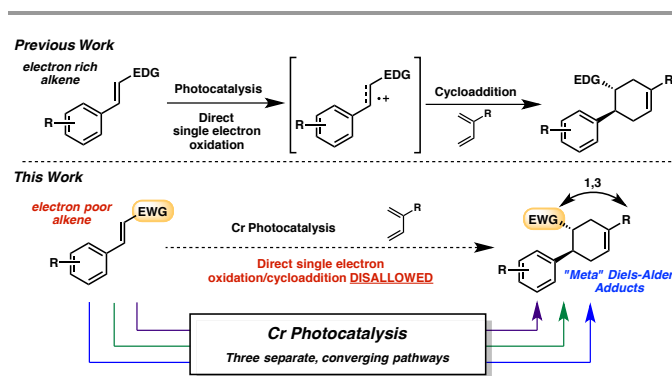
Fig. 1. Photocatalyzed [4+2] cycloadditions with electron deficient alkenes.
