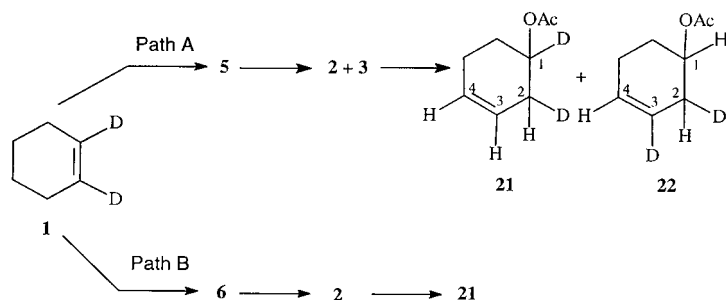
Scheme 6. Expected outcome of the oxypalladation route (A) versus the ( \pi -allyl) route (B) in the homoallylic acetoxylation of 1,2-dideuteriocyclohexene.
