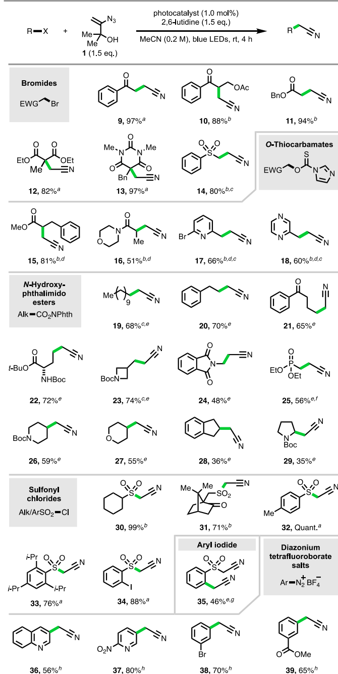
Scheme 3 Cyanomethylation of radicals. Reaction conditions: all reactions run on a 1.0 mmol scale; a Ru(bpy) 3 Cl 2 ·6H 2 O; b fac -Ir(ppy) 3 ; c 24 h; d no 2,6-lutidine; e Ir(5-Fppy) 3 , (+)-sodium L-ascorbate (1.5 eq.); f no (+)-sodium L-ascorbate; g 8 h; h no photocatalyst, no LEDs.
