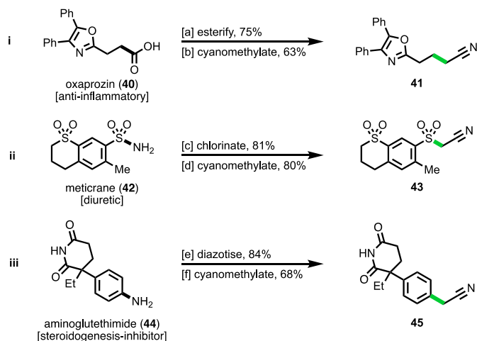
Scheme 4 Late-stage cyanomethylation of pharmaceuticals. Reaction conditions: a oxaprozin ( 40 ), PhthNOH, DCC, DMAP, CH 2 Cl 2 , rt, 16 h; b N -hydroxyphthalimido ester ( 1 ) (1.5 mmol), Ir( 1 ) (1.5 mmol), Ir( 1 ) (0.01 mmol), DMSO (0.2 M), blue LEDs, rt, 24 h; c metircane ( 42 ), ClSO 3 H, 100 °C, 2 h; d sulfonyl chloride ( 1 ) (1.5 mmol), 2,6-lutidine (1.5 mmol), Ru(bpy) 3 Cl 2 ·6H 2 O (0.01 mmol), MeCN (0.2 M), blue LEDs, rt, 4 h; e aminogluthethimide ( 44 ), NaNO 2 , aq. HBF 4 , H 2 O, 0 °C, 30 min; f Diazonium salt ( 1 ) (1.5 mmol), 2,6-lutidine (1.5 mmol), MeCN (0.2 M), rt, 4 h.
