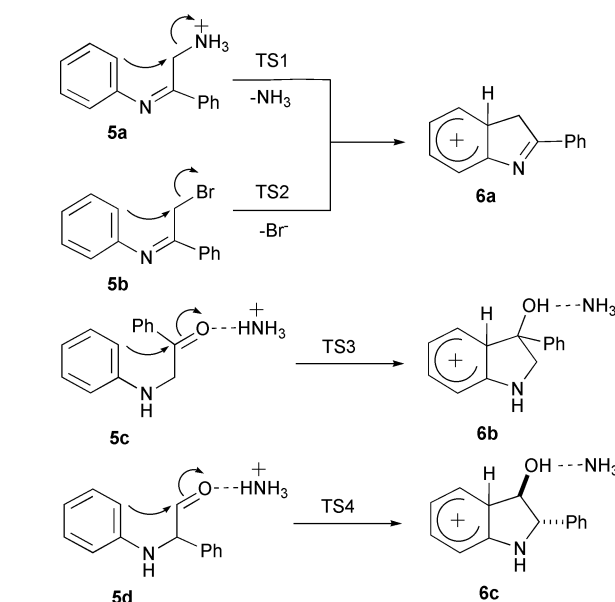
Scheme 5 Model cyclization steps computed at the B3LYP/6-31G* level.
