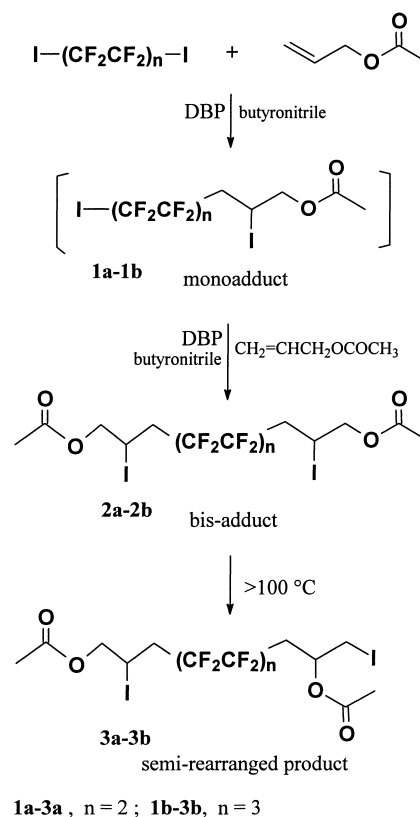
Scheme 1. Products of radical addition of diiodoperfluoroalkanes to allyl acetate.
