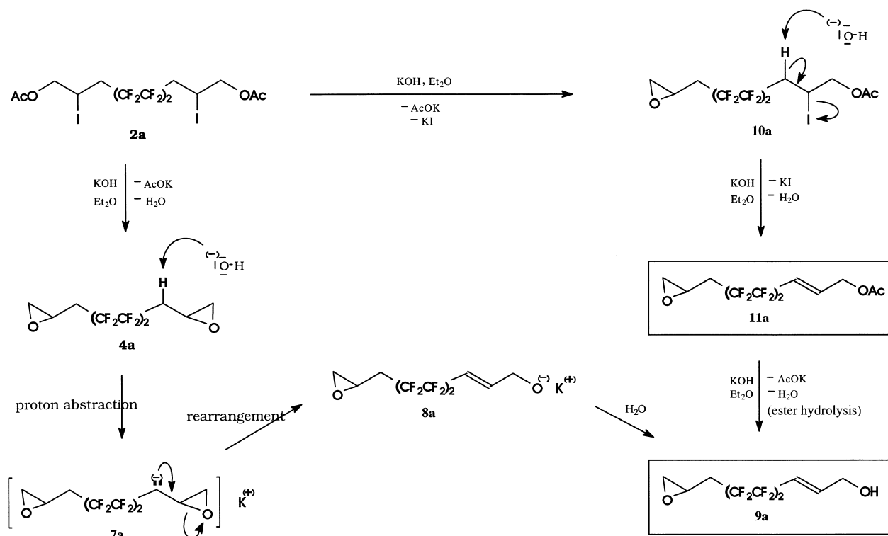
Scheme 3. Probable reaction sequence in the formation of by-products in the epoxidation of adducts 2a–2b and 3a–3b .
