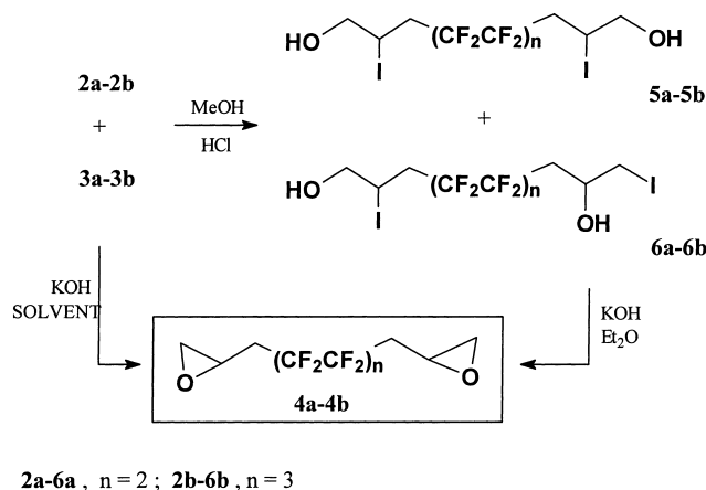
Scheme 2. Preparation of diepoxides 4a–4b from bis-adducts 2a–2b and rearranged bis-adducts 3a–3b .
