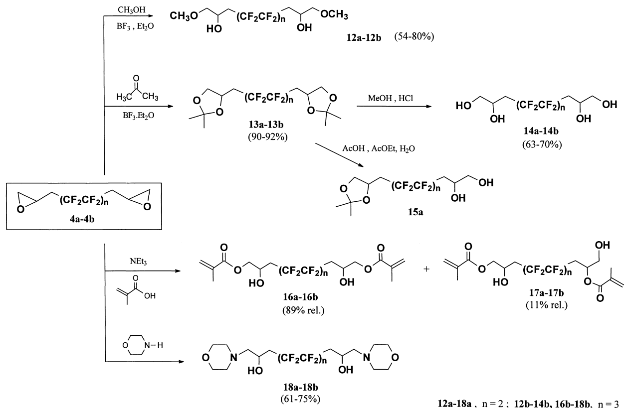
Scheme 4. Nucleophilic reactions of diepoxides 4a-4b .
