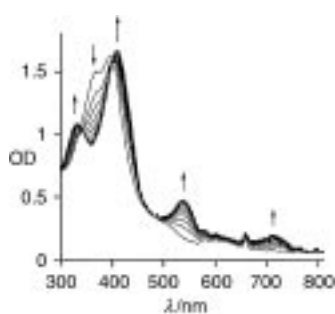
Figure 7. Spectral changes upon the reduction of [Fe(tpfc)Cl] ( 5b ) at 200 mV ( \text{CH}_2\text{Cl}_2 , 0.1M TBAP).
