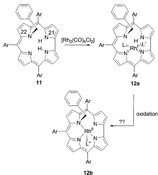
Scheme 4. Rhodium insertion into \text{H}_2(\text{N}^{22}\text{-benz-tpfc}) ( 11 ) to form 12a (see Figure 5 for its X-ray structure) and its plausible oxidation product 12b ( \text{L} = \text{CO} , \text{L}' = \text{PPh}_3 , \text{L}'' = \text{CO} or \text{PPh}_3 ).
