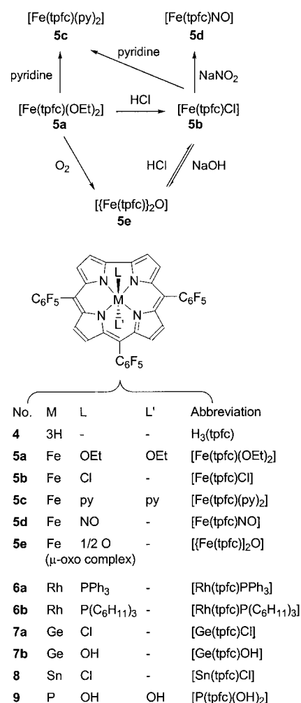
Scheme 2. Formulae of 5,10,15-tris(pentafluorophenyl)corrole and its metal complexes, and the interconversion of the various iron corroles.
