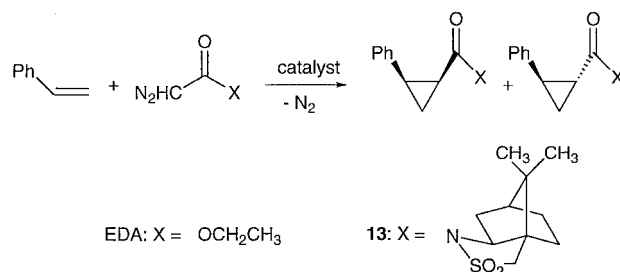
Scheme 5. Metallo-corrole-catalyzed cyclopropanation of styrene by carbenoids.
