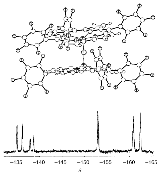
Figure 3. The X-ray structure [[Fe(tpfc)] 2 O] ( 5e ) and its 19 F NMR spectrum (25 °C, [D 6 ]benzene).
