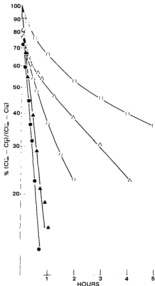
Figure 3 —The effect of pH on the hydrolysis of I (0.35 mg/ml) as determined by chloride titration. All pHs (apparent) are with sodium citrate buffer ( 4.2 \times 10^{-2} M). Key: (□) pH 3.0; (Δ) pH 3.5; (○) pH 4.0; (▲) pH 5.0; (●) pH 6.0.
