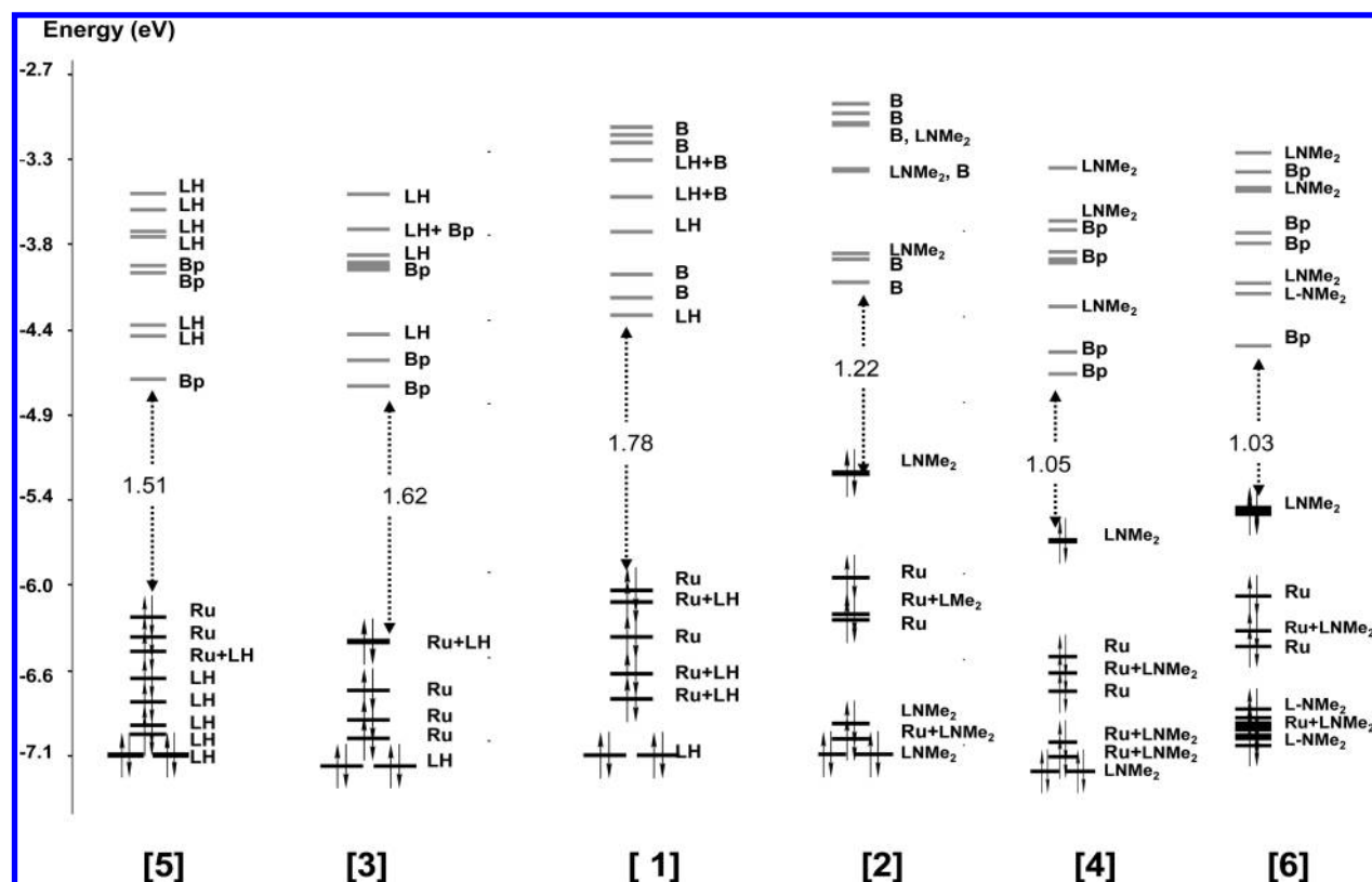
Figure 3. Molecular orbital diagram for ruthenium complexes (Ru = ruthenium; B = bipyridine; Bp = dimethyl dicarboxylate of bipyridine; LH = 4,4'-distyryl-2,2'-dipyridine; LNMMe 2 = 4,4'-bis[ p -(dimethylamino)- \alpha -styryl]-2,2'-bipyridine).
