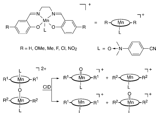
Scheme 2. Possible fragmentation products upon CID of \mu -oxomanganese(IV)–salen complexes with salen ligands with different substituents in the 5- and 5'-positions.
