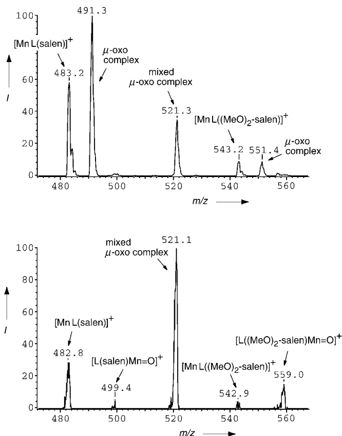
Figure 2. Top: electrospray mass spectrum of a solution of [Mn((MeO) 2 –salen)]ClO 4 , [Mn(salen)]ClO 4 , p -CN- N,N -dimethylaniline N -oxide, and iodosobenzene in acetonitrile, and this shows the formation of homogeneous and mixed \mu -oxo complexes with terminal N -oxide ligands; bottom: daughter-ion spectrum (0.09 Pa Ar, collision energy 34 eV) of the mixed dinuclear complex [L((MeO) 2 –salen)Mn–O–Mn(salen)L] 2+ ( m/z : 521, L = p -CN- N,N -dimethylaniline N -oxide), and this shows both the fragmentation to [MnL((MeO) 2 –salen)] + ( m/z : 543) and to the corresponding oxo complex ( m/z : 559).
