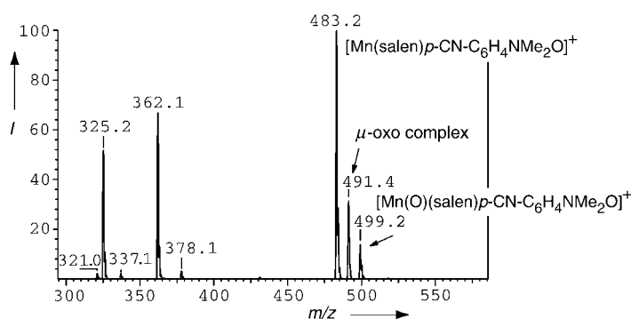
Figure 1. Electrospray mass spectrum of a solution of [\text{Mn}(\text{salen})]\text{ClO}_4 , p\text{-CN}-N,N -dimethylaniline N -oxide, and iodosobenzene in acetonitrile; this shows the formation of N -oxide ligated manganese(III) and oxomanganese species.
