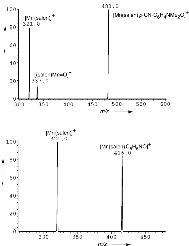
Figure 6. Top: daughter-ion spectrum (0.13 Pa Ar, collision energy 20 eV) of [p\text{-CN-C}_6\text{H}_4\text{NMe}_2\text{O-Mn}^{\text{III}}(\text{salen})]^+ , and this shows fragmentation of the Mn–O as well as of the N–O bond; bottom: daughter-ion spectrum (0.13 Pa Ar, collision energy 20 eV) of [\text{Mn}^{\text{III}}(\text{pyO})(\text{salen})]^+ , and this shows exclusive loss of pyridine N -oxide.
