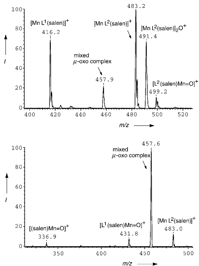
Figure 5. Top: electrospray mass spectrum of a solution of [\text{Mn}(\text{salen})]\text{-ClO}_4 and iodosobenzene with pyridine N -oxide and p -CN- N,N -dimethylaniline N -oxide in acetonitrile; bottom: daughter-ion spectrum (0.08 Pa Ar, collision energy 14 eV) of the dinuclear \mu -oxo complex [\text{L}^1(\text{salen})\text{Mn-O-Mn}(\text{salen})\text{L}^2]^+ ( m/z : 457.5, \text{L}^1 = pyridine N -oxide, \text{L}^2 = p -CN- N,N -dimethylaniline N -oxide), and this shows exclusive fragmentation to [\text{MnL}^2(\text{salen})]^+ ( m/z : 483) and to the oxo complex [\text{L}^1(\text{salen})\text{Mn=O}]^+ ( m/z : 432).
