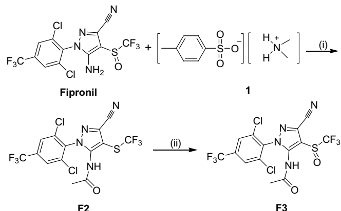
Scheme 1. Reagents and conditions: (i) \text{CH}_3\text{COCl} , \text{CH}_2\text{Cl}_2 , reflux (35%); (ii) mCPBA, rt, \text{CH}_2\text{Cl}_2 (70%).
