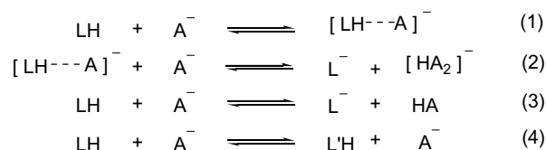
Fig. 1. The possible equilibria of \text{LH} and \text{A}^- .
