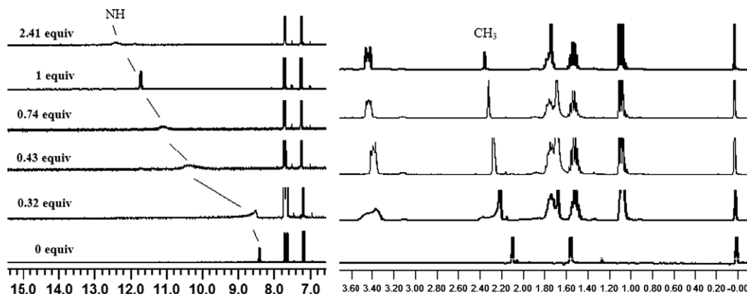
Fig. 5. ^1\text{H} NMR titration of F3 with tetrabutylammonium chloride in \text{CDCl}_3 at 298 K [\text{F3}] = 8.0 \times 10^{-3} \text{ M} , [\text{Cl}^-] = 0\text{--}2.0 \times 10^{-2} \text{ M} .
