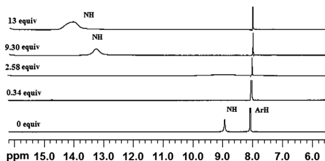
Fig. 4. ^1\text{H} NMR spectra of F3 with tetrabutylammonium acetate in \text{CD}_3\text{CN} at 298 K (only NH and aromatic protons are shown) [\text{F3}] = 8.0 \times 10^{-3} \text{ M} , [\text{AcO}^-] = 0\text{--}2.0 \times 10^{-2} \text{ M} .
