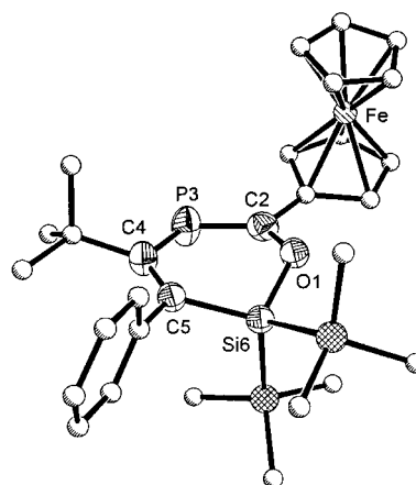
Figure 2. Molecular structure of 20b in the solid state. Selected bond lengths [Å] and angles [ ^\circ ]: P3–C2 1.678(4), C2–O1 1.339(3), O1–Si6 1.692(2), Si6–C5 1.866(4), C5–C4 1.336(4), C4–P3 1.845(2); C4–P3–C2 105.5(1), P3–C2–O1 129.1(2), C2–O1–Si6 117.5(2), O1–Si6–C5 105.0(1), Si6–C5–C4 119.4(2), C5–C4–P3 123.0(3).
