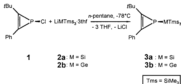
Scheme 1. Synthesis of the 1-silyl- and 1-germyl-1 H -phosphirenes 3a and 3b .
