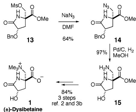
Scheme 5. Completion of Total Synthesis of (±)-Dysibetaine ( 1 )
