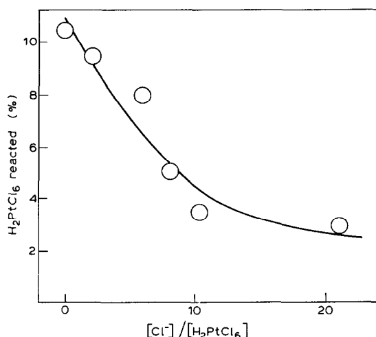
Fig. 11. Plot of the conversion of \text{PtCl}_6^{2-} in the photoinduced reaction of \text{H}_2\text{PtCl}_6 (0.02 M ) with styrene (0.17 M ) in \text{CH}_3\text{COOH} for 6 min versus concentration of LiCl added (relative to [\text{PtCl}_6^{2-}] ).
