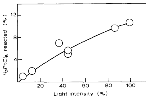
Fig. 10. Plot of the conversion of \text{PtCl}_6^{2-} in the photoinduced reaction of \text{H}_2\text{PtCl}_6 (0.02 M ) with styrene (0.17 M ) in \text{CH}_3\text{COOH} for 6 min versus light intensity (full light of a high-pressure mercury lamp was 100%).
