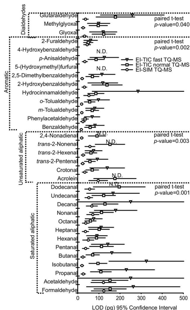
Figure 5. Comparison of LODs in pg (graphically depicted as circles, squares, and triangles) with their 95% confidence interval (graphically depicted as lines) for EI-SIM-TQ-MS (open circle), EI(n-TIC)-TQ-MS (open square), and EI(f-TIC)-TQ-MS (inverted open triangle). Tabulated LOD intervals for all aldehydes and modes of acquisition are provided in the supplementary Table S2. Confidence intervals may be directly related to a method precision at low detection levels. Two-tail paired t -test P value shows whether there is a significant difference in sensitivity between EI(n-TIC)-TQ-MS and EI(SIM)-TQ-MS for a group of aldehydes (saturated and unsaturated aliphatic, aromatic, and dialdehydes), the lower P value the greater probability that methods are different. N.D. = not detected within the tested range of 50–600 pg.
