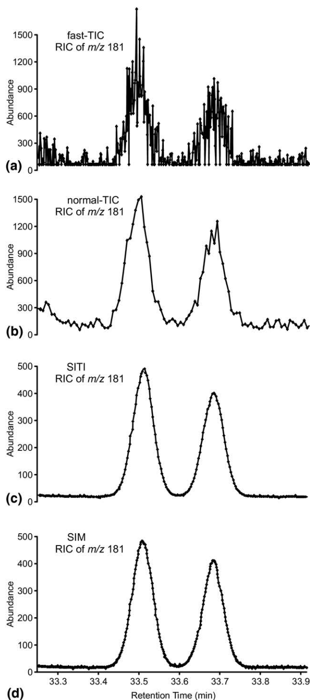
Figure 6. The reconstructed ion chromatograms (RIC) of m/z of 181 of heptanal ( syn/anti stereoisomers) acquired using (a) EI(f-TIC)-TQ-MS, (b) EI(n-TIC)-TQ-MS, (c) EI(SITI)-TQ-MS, where SIM signal was used, and (d) EI(SIM)-TQ-MS. The peak half-widths were ~6 s; f-TIC (a) provided ~100, n-TIC (b) ~21, SITI (c) ~40, and SIM (d) ~70 data points across the chromatographic peak. A low signal-to-noise ratio in (a) caused the decrease of detectability and reproducibility compared with (b). SITI (c) and SIM (d) had similar signal-to-noise ratio, thus the detectability and reproducibility (peak shape) of the two scanning methods were comparable. The amount of analyte was 150 pg, which was near LOD in TIC mode.
