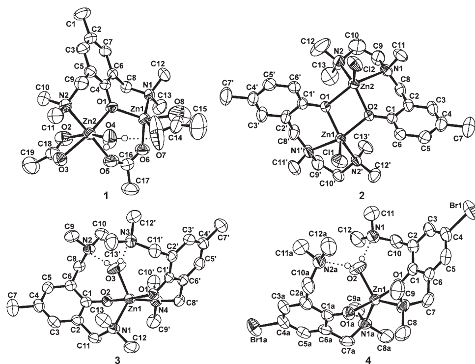
Figure 3. X-ray crystal structures of 1 – 4 . In 1 , the water molecule is hydrogen bonded to one of the acetate ligands, whereas in 3 and 4 , the water molecules are hydrogen bonded to the tertiary amino substituents. The hydrogen atoms (except those of water molecules) are omitted for clarity.
