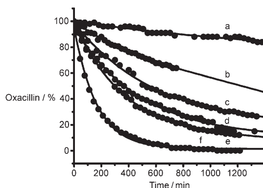
Figure 5. Hydrolysis of oxacillin ( 1.06 \times 10^{-3} M) by a) HL 1 , b) zinc acetate, c) 4 , d) 3 , e) 2 , f) 1 (each 2.1 \times 10^{-5} M) in DMSO/HEPES buffer (1:9), pH 7.5. The reaction was monitored by reverse-phase HPLC and the amount of oxacillin hydrolyzed at any given time was calculated from the calibration plot.
