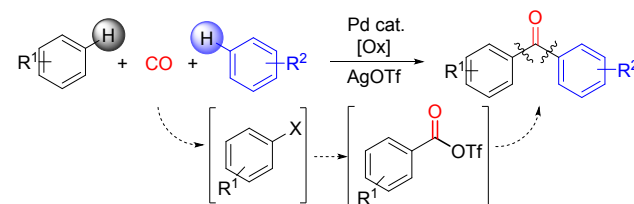
Figure 1 Approaches to Intra- and Intermolecular Oxidative C-H Functionalization and Application to Ketone Synthesis.
