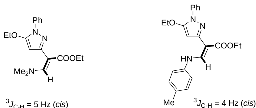
Figure 1. Determination of configuration around the \text{C}=\text{C} double bonds by NMR spectroscopy.
