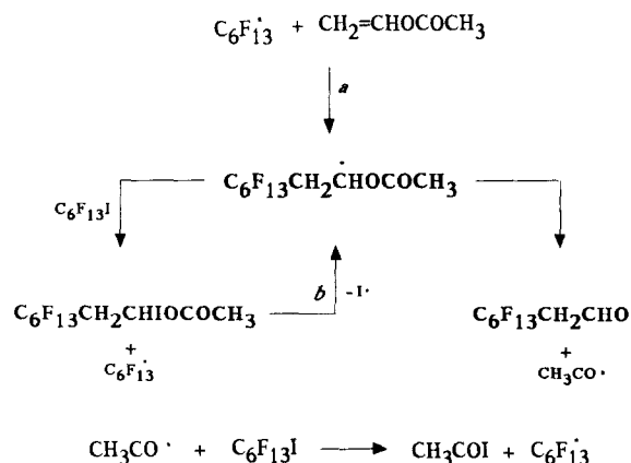
Fig. 3. Possible mechanisms for aldehyde formation during the radical addition step.
