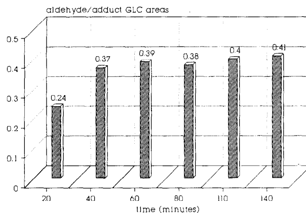
Fig. 2. Aldehyde/adduct GLC areas ratio versus time in the radical addition step.
