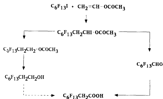
Fig. 1. Outline of the perfluorohexyl acetic acid synthesis using (a) the modified method and (b) the previous method. The dashed line refers to the oxidation step (not reported in ref. 5) of the alcohol to the corresponding carboxylic acid.
