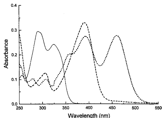
Figure 1. Electronic absorption spectra of 6dH (—), 14bH (---), and 15 (.....) in \text{CH}_3\text{CN} ( 10^{-5} M) at 25^\circ\text{C} .
