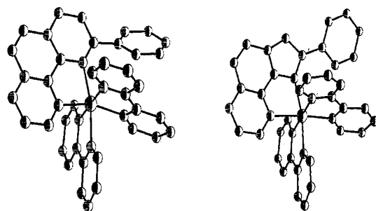
Figure 2. Molecular mechanics simulation of [\text{Ru}(\text{L})(\text{bpy})_2]^{2+} (left) and [\text{Ru}(\text{6b})(\text{bpy})_2]^+ (right) where L = 2-phenyl-1,10-phenanthroline.
