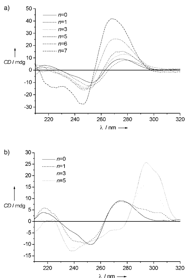
Figure 5. CD spectra of selected duplexes from Table 1. Top: base I, n = 0, 1, 3, 5, 6, 7 ; c = 3.6 \mu\text{M} in 10 mM \text{NaH}_2\text{PO}_4 , 0.15 M NaCl, pH 7, T = 20^\circ\text{C} ; bottom: base Y, n = 0, 1, 3, 5 . c = 3.6 \mu\text{M} in 10 mM \text{NaH}_2\text{PO}_4 , 0.15 M NaCl, 1 mM EDTA, pH 7, T = 20^\circ\text{C} .
