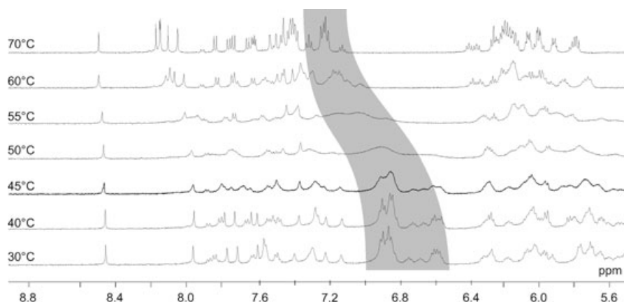
Figure 4. Temperature dependent ^1\text{H} NMR spectra (500 MHz) of the DNA duplex 5'd(GATGACIGCTAG)-d(CTAGCIGTCATC) ( c = 1 mM, 10 mM \text{NaH}_2\text{PO}_4 , 150 mM NaCl, pH 7, 100% \text{D}_2\text{O} ).
