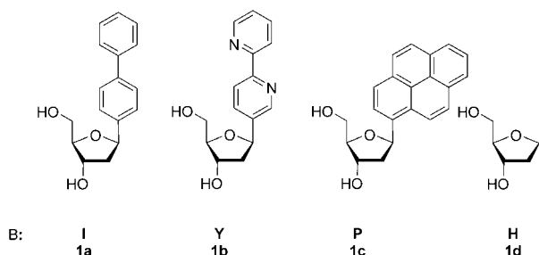
Figure 1. Chemical structures of the hydrophobic nucleosides used in this study.
