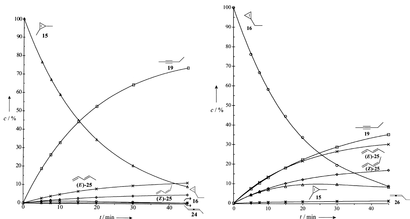
Figure 1. Time evolution of the decomposition of 15 at 248.4°C (left) and of 16 at 238.6°C (right).
