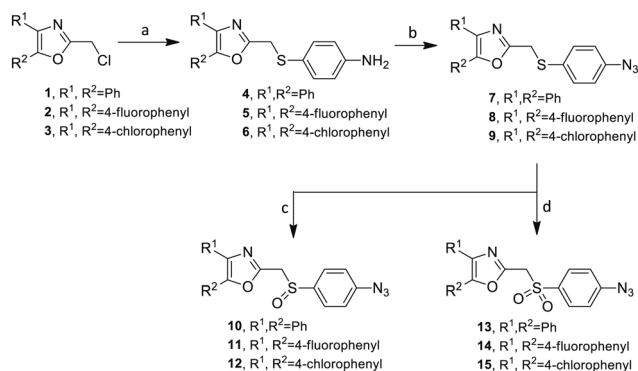
Scheme 1 Synthesis of azidophenylsulfinyl and azidophenylsulfonyl click partners 10–15. Reagents/conditions: (a) NaH/4-aminothiophenol/THF/0–5 °C to rt/16 h (66–85%). (b) NaNO 2 /10% HCl/NaNO 3 /0–5 °C to rt/16 h (61–98%). (c) MCPBA (1.2 equiv.)/DCM/rt/16 h (86–95%). (d) MCPBA (3 eq.)/DCM/rt/16 h (86–93%).
