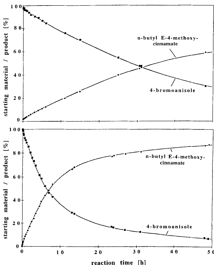
Figure 2. Concentration versus time diagram (GLC) for the Heck-olefination of 4-bromoanisole (as an example of a deactivated bromoarene) with n -butyl acrylate at T = 140^\circ\text{C} . For reaction conditions, see Table 1. The decrease in 4-bromoanisole (■) (reactant) and increase in n -butyl ( E )-4-methoxycinnamate (●) (Heck product) is shown. Top: “in situ catalyst” [\text{Pd}(\text{OAc})_2]/\text{P}(\textit{o}\text{-Tol})_3 with \text{Pd}:\text{P} = 1:1 (1 mol % Pd); bottom: palladacycle 1a as catalyst (1 mol % Pd).
