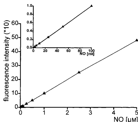
Figure 6. Dependency of the fluorescence intensity of 6c on the NO concentration after reaction with 4c ( c = 50\text{ }\mu\text{M} , \lambda_{\text{exc}} = 380\text{ nm} , \lambda_{\text{em}} = 460\text{ nm} ) for the micromolar and nanomolar range in sodium phosphate buffer pH 7.2.
