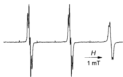
Figure 3. ESR spectrum of 5c . Radical 5c was generated in THF solution by reaction of 4c with NO at 23 °C. ESR parameters: g = 2.00610 , a(^{14}\text{N}) = 2.287 \text{ mT} , a(\text{exo-H}_\gamma) = 0.076 \text{ mT} (2H), a(\text{H}) = 0.048 \text{ mT} (1H), a(\text{H}) = 0.014 \text{ mT} (4H).
