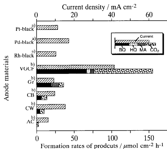
Figure 1. Oxidation of benzene over various anodes during \text{H}_2\text{O} electrolysis at 298 K. Reaction time 2 h, \text{H}_3\text{PO}_4 1 mol/l, benzene 40 ml. Anode potential (Ag|AgCl); a) 1.5 V, b) 2.0 V. BQ benzoquinone, HQ hydroquinone, MA maleic acid.
