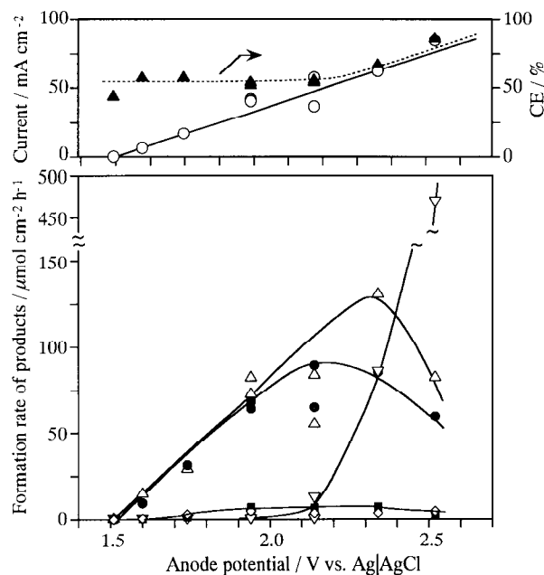
Figure 2. Effects of applied voltage on the oxidation of benzene over the VGCF anode at 298 K. Reaction time 2 h, \text{H}_3\text{PO}_4 1 mol/l, benzene 40 ml. BQ ●, HQ ■, MA ◇, \text{CO}_2 △, \text{O}_2 ▽, current ○, current efficiency (BQ+HQ+MA+ \text{CO}_2 + \text{O}_2 ) ▲.
