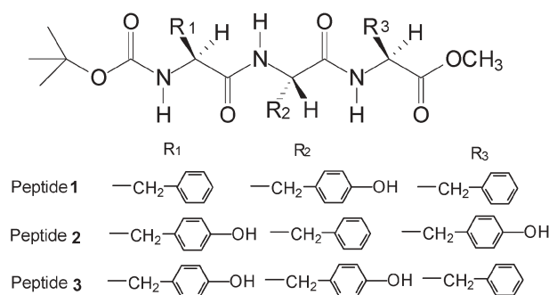
Fig. 1 Schematic representation of tripeptides 1, 2 and 3 showing their chemical structures.
