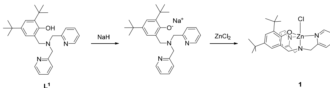
Scheme 1. Synthesis of 1 .
