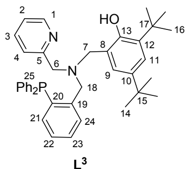
Figure 14: [L^3]H with position numbering.
