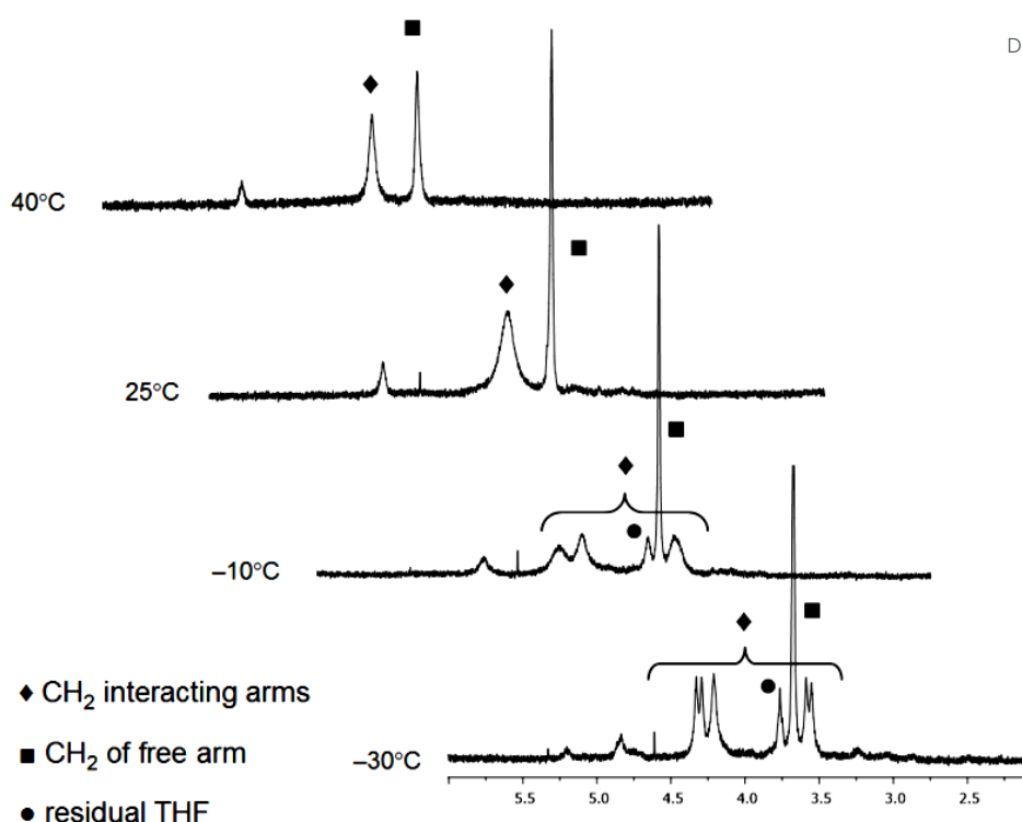
Figure 9. Variable temperature ^1\text{H} NMR experiment for (\text{L}^5)\text{ZnCl}_2 ( 5 ); benzylic region (400 MHz, from 40^\circ\text{C} to -30^\circ\text{C} , \text{CDCl}_3 ).
