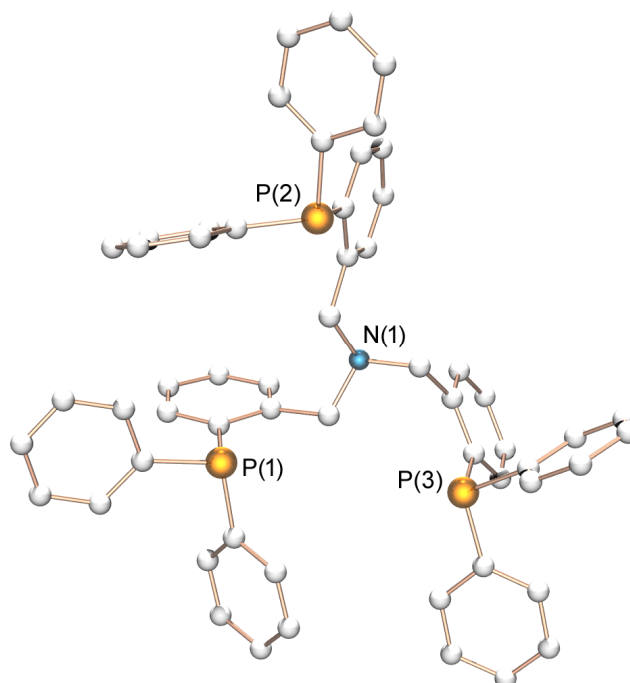
Figure 5. Molecular structure of tripodal pro-ligand L^5 (hydrogen atoms are omitted for clarity)
