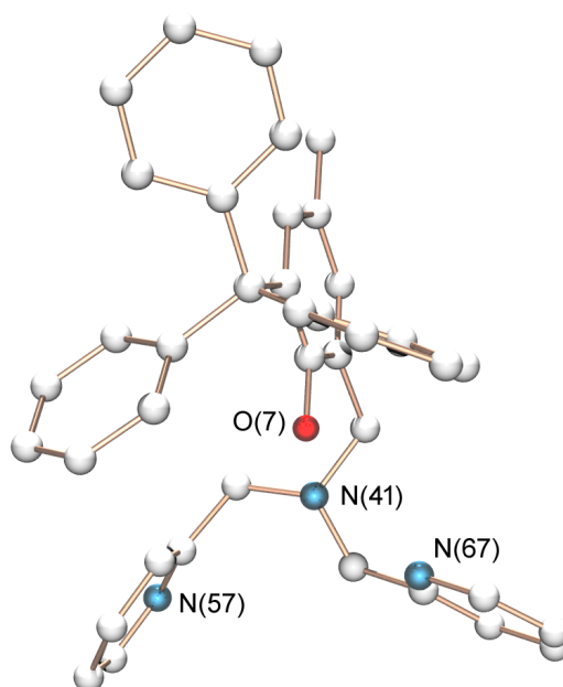
Figure 3. Molecular structure of pro-ligand [L 2 ]H (hydrogen atoms and solvent molecules are omitted for clarity)
