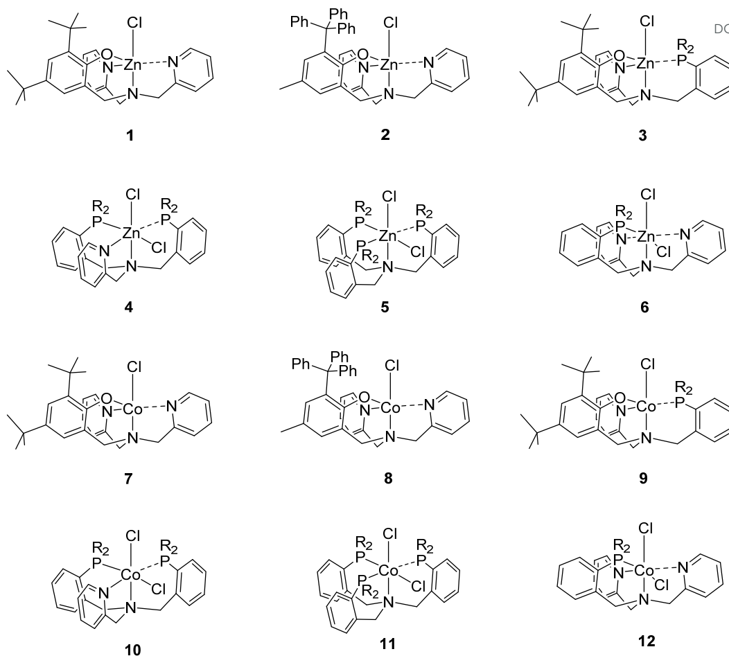
Figure 7. Complexes 1-12 (R = Ph).
