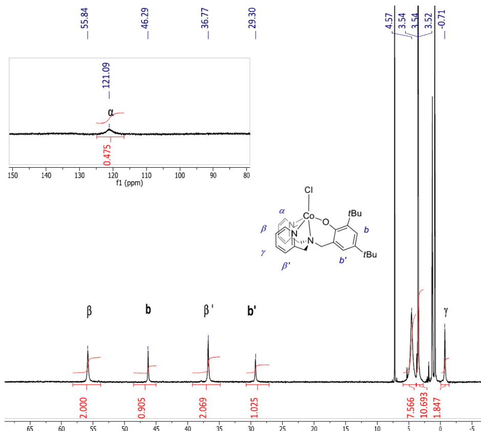
Figure 12. ^1\text{H} NMR spectrum of complex 7 ( \text{CDCl}_3 , 25^\circ\text{C} , 300 MHz).
