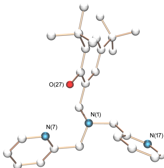
Figure 2. Molecular structure of pro-ligand [L 1 ]H (hydrogen atoms and solvent molecules are omitted for clarity)
