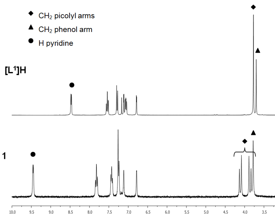
Figure 8. ^1\text{H} NMR spectra of pro-ligand [\text{L}^1]\text{H} (up) and 1 (down) ( \text{CDCl}_3 , 25^\circ\text{C} , 300 MHz).
