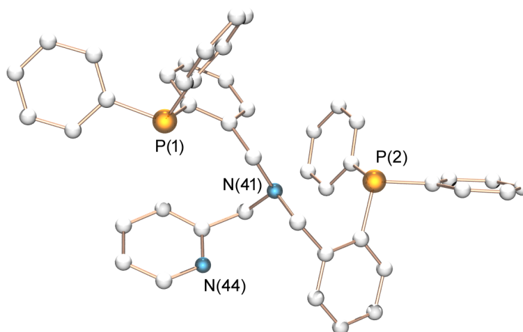
Figure 4. Molecular structure of pro-ligand L^4 (hydrogen atoms are omitted for clarity)
