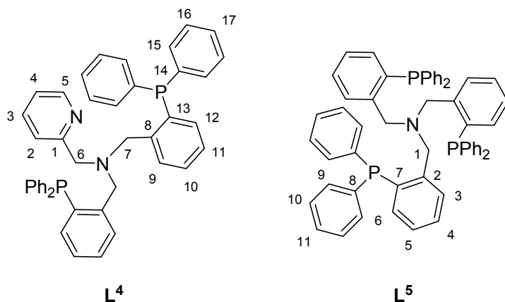
Figure 15: \text{L}^4 and \text{L}^5 with position numbering.
