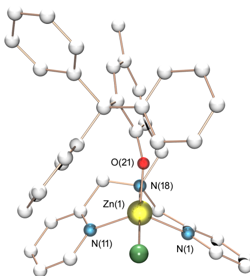
Figure 10. Molecular structure of 2 (hydrogen atoms and solvent molecule are omitted for clarity).
