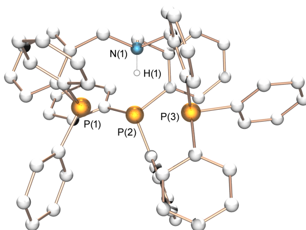
Figure 6. Molecular structure of tripodal ammonium salt L^5 \cdot HCl (hydrogen atoms and chloride anion are omitted for clarity)
