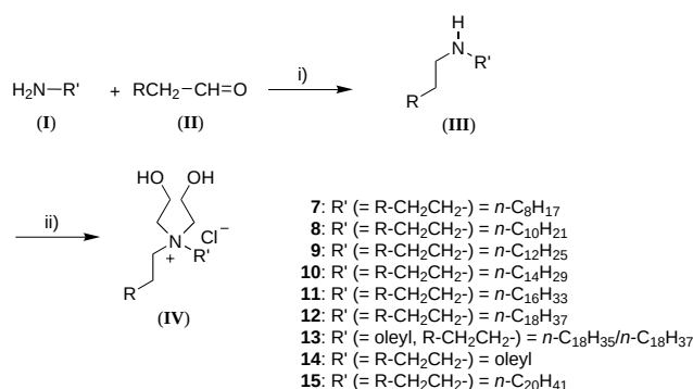
Scheme 2. Syntheses of new DHDEAB analogues. i) MgSO 4 (1 equiv), dichloromethane; ii) NaBH 4 (2 equiv), dichloromethane/MeOH; ii) excess chloroethanol/aqueous NaOH.
