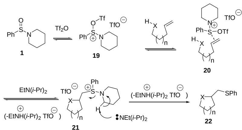
Scheme 1. Mechanism for Cyclization with BSP/Tf 2 O.
