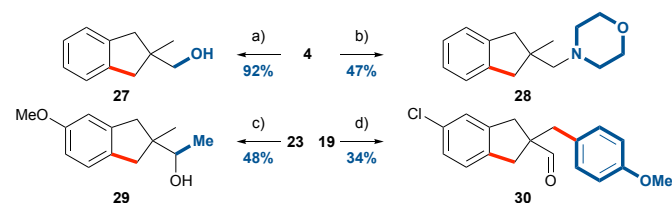
Scheme 3: Derivatisation of indane products. a) NaBH 4 , MeOH, 2 h 0–25 °C, b) morpholine, NaBH(OAc) 3 , CH 2 Cl 2 , 25 °C, 24 h. c) MeMgCl, Et 2 O, 0–25 °C, 1.5 h. d) TDG1 (50 mol%), 4-iodoanisole, Pd(OPiv) 2 (5 mol%), AgTFA, DMSO (1 equiv), HFIP:AcOH (1:1), 130 °C, 3 h. Product isolated as a 5.7:1 mixture with a 4-acetoxyanisole by-product.
