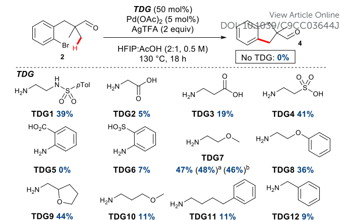
Scheme 2: Screen of transient directing groups for C-H annulation, indicating the yield of indane 4 . *25 mol% TDG7 . b 1 equiv TDG7 .
