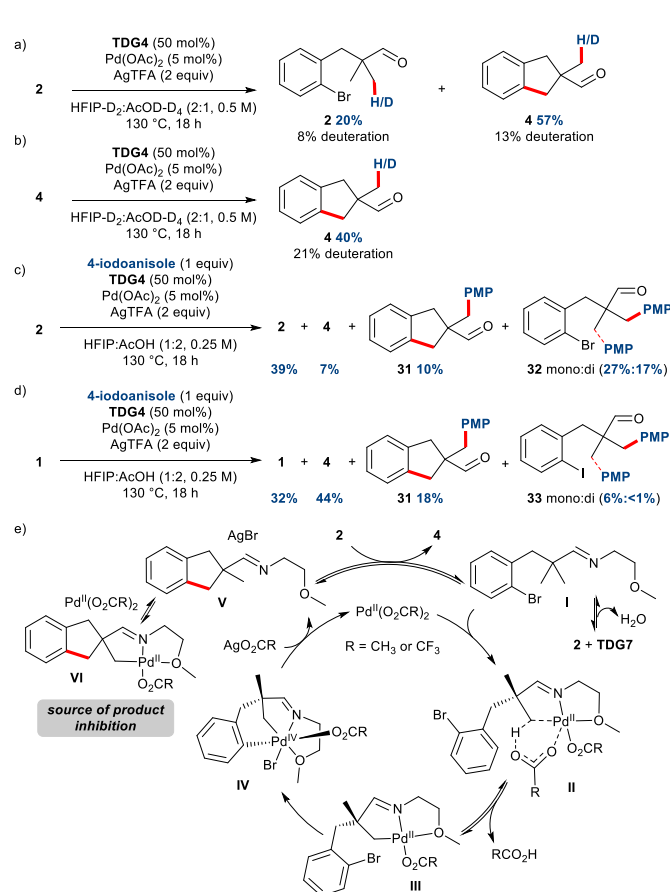
Scheme 4: Mechanistic experiments. a) Deuteration experiment showed small levels of deuteration in RSM 2 and indane 4 , yields determined by 1 H NMR using 1,3,5-trimethoxybenzene as an internal standard. b) Deuteration of indane 4 , yields determined by 1 H NMR using 1,3,5-trimethoxybenzene as an internal standard. Competition experiments with c) external aryl iodide and internal aryl bromide, and d) external aryl iodide and internal aryl iodide, values given are conversions. e) Proposed catalytic cycle.
