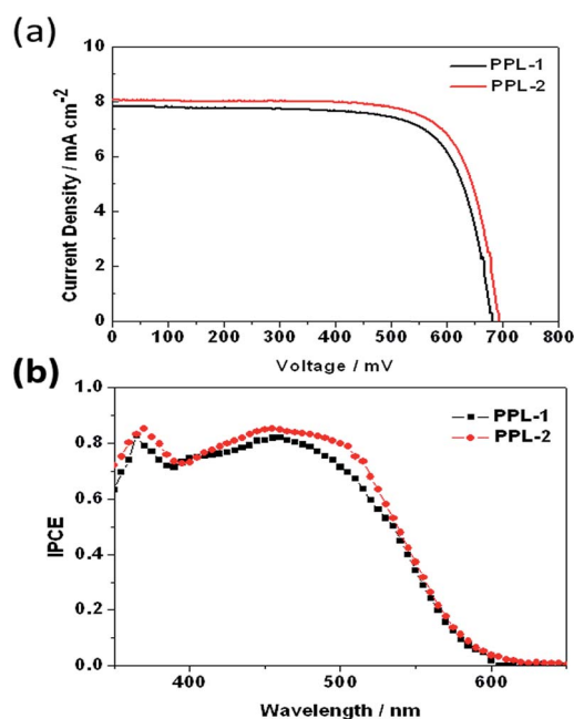
Fig. 2 Photocurrent density-voltage ( J - V ) curves (a), and incident photon-to-current conversion efficiency (IPCE) (b) spectra of DSCs for PPL-1 and PPL-2.
