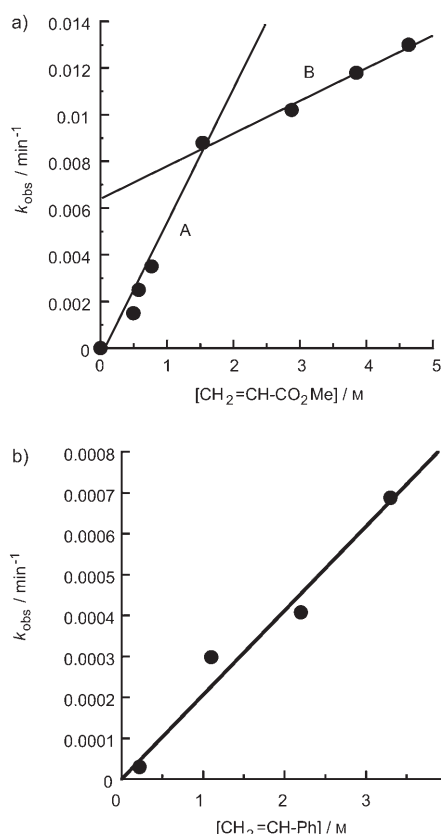
Figure 4. Kinetics of the reaction of [Pd(dppp)IPh] ( 2b ) in dmf at 25°C with a) methyl acrylate and b) styrene. Determination of the reaction order in alkenes: plot of k_{obs} against alkene concentration.
