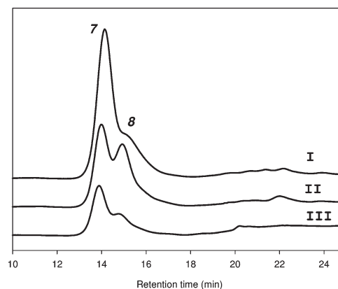
Figure 4. HPLC chromatograms showing the formation of the two mono-stearates of resveratrol using (I) lipase QLG; (II) lipase PS IM; and (III) lipase TL IM. Screening conditions: 50 mM resveratrol, 750 mM vinyl stearate, 150 mg/mL biocatalyst, and 40 °C. The chromatograms correspond to a reaction time of 138 h.
