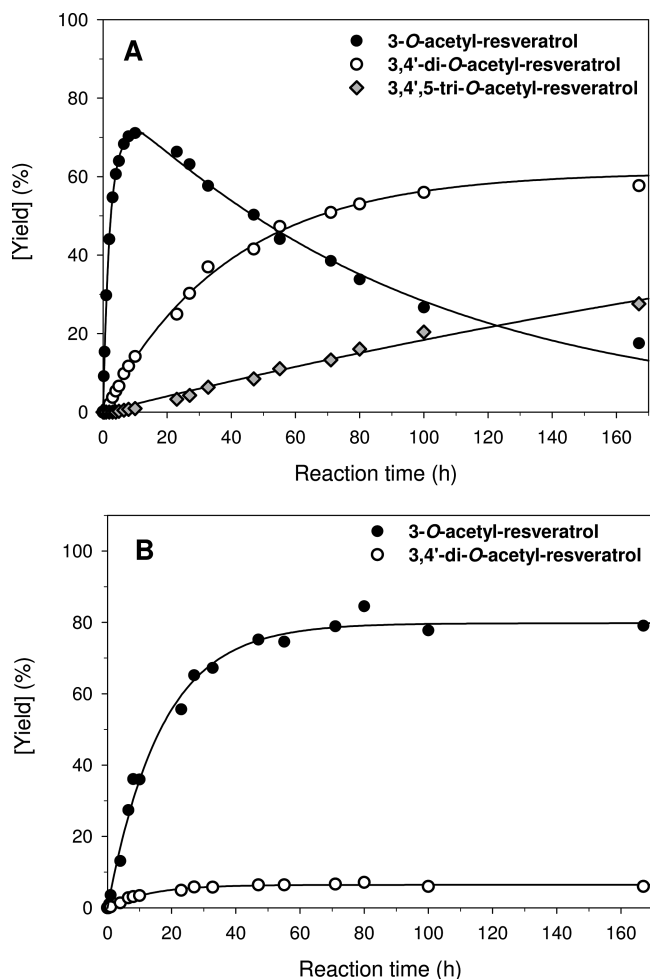
Figure 3. Kinetics of resveratrol acetylation in 2M2B catalyzed by (A) lipase QLG and (B) Novozym 435. Experimental conditions: 50 mM resveratrol, 750 mM vinyl acetate, 150 mg/mL biocatalyst, and 40 °C.
