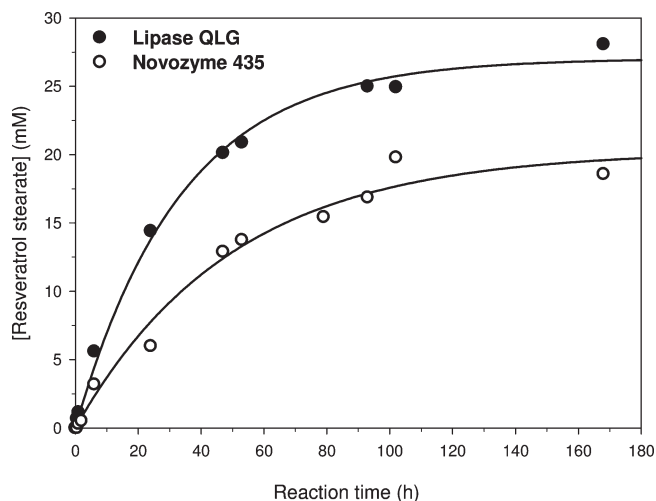
Figure 5. Kinetics of resveratrol acylation with vinyl stearate in 2M2B catalyzed by lipase QLG and Novozyme 435. Experimental conditions: 50 mM resveratrol, 750 mM vinyl stearate, 150 mg/mL biocatalyst, 150 rpm, and 40 °C.
