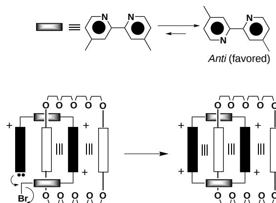
Figure 1. Schematic illustration of a possible route for the formation of the catenanes 8 ·4PF 6 and 9 ·4PF 6 .
