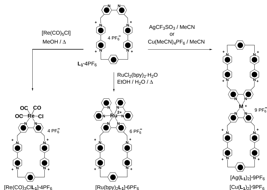
Scheme 3. Preparation of the mononuclear \text{Ag}^{\text{I}} , \text{Cu}^{\text{I}} , \text{Re}^{\text{I}} , and \text{Ru}^{\text{II}} complexes containing the cyclophane \mathbf{L}_1^{4+} .
