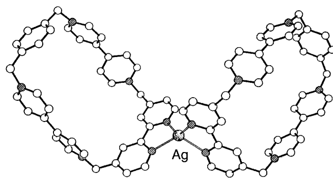
Figure 4. X-ray crystal structure of the complex [\text{Ag}(\text{L}_1)_2](\text{PF}_6)_9 .
