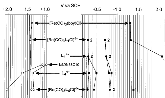
Figure 11. Genetic diagram of the redox potentials of the \text{L}_1^{4+} cyclophane ligand, the \text{L}_4^{4+} catenane ligand, and of their \text{Re}^{\text{I}} complexes. For comparison purposes, the redox potentials of the [\text{Re}(\text{CO})_3(\text{Cl})(\text{bpy})] model compound and of the crown ether 1/5DN38C10, which is a component of \text{L}_4^{4+} , are also shown. Solid symbols correspond to reduction processes centered on the paraquat- (●) and the bipyridine-type (■) units. Empty symbols correspond to oxidation processes centered on the \text{Re}^{\text{I}} metal ion (○) and the 1/5DMN units (○).
