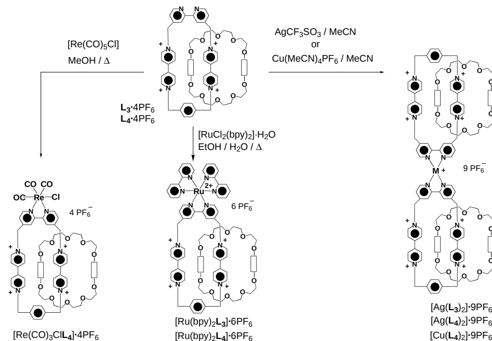
Scheme 4. Preparation of the mononuclear \text{Ag}^{\text{I}} , \text{Cu}^{\text{I}} , \text{Re}^{\text{I}} , and \text{Ru}^{\text{II}} complexes containing the [2]catenanes \mathbf{L}_3^{4+} and \mathbf{L}_4^{4+} .
