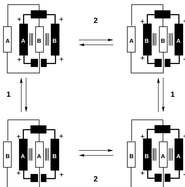
Scheme 6. The dynamic processes occurring in the [2]catenanes L_3^{4+} and L_4^{4+} on the ^1H NMR time scale.
