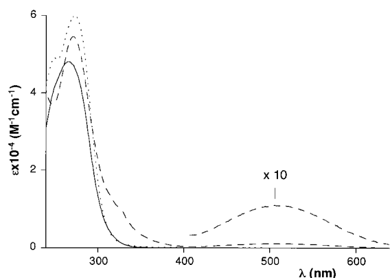
Figure 8. Absorption spectra (MeCN, 298 K) of the ligands \mathbf{L}_1^{4+} (full line), \mathbf{L}_2^{4+} (dotted line), and \mathbf{L}_4^{4+} (dashed line).
