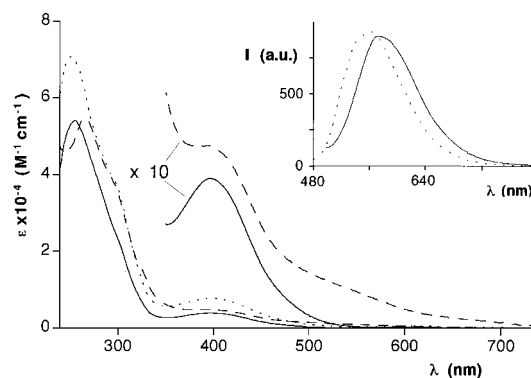
Figure 9. Absorption (MeCN, 298 K) and luminescence (inset: butyronitrile, 77 K) spectra of the complexes [\text{Re}(\text{CO})_3\mathbf{L}_1\text{Cl}]^{4+} (full line), [\{\text{Re}(\text{CO})_3\text{Cl}\}_2\mathbf{L}_2]^{4+} (dotted line), and [\text{Re}(\text{CO})_3\mathbf{L}_4\text{Cl}]^{4+} (dashed line).
