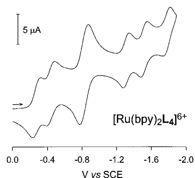
Figure 12. Cyclic voltammetric behavior on reduction of 5 \times 10^{-4} M [\text{Ru}(\text{bpy})_2\text{L}_4]^{6+} (acetonitrile solution, 298 K, potential values vs. SCE, scan rate 50 \text{ mV s}^{-1} , glassy carbon as working electrode, 0.05 \text{ M Et}_4\text{NPF}_6 as supporting electrolyte).
