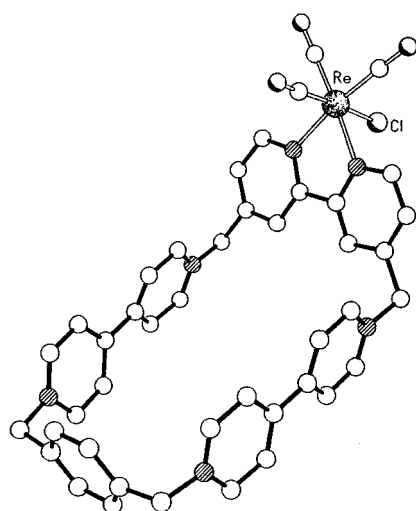
Figure 3. X-ray crystal structure of the complex [\text{Re}(\text{CO})_3\text{L}_1(\text{Cl})](\text{PF}_6)_4 .
