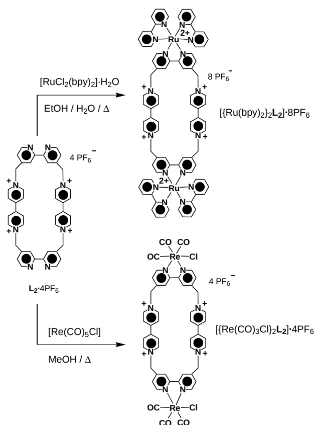
Scheme 5. Preparation of the binuclear Re^I and Ru^{II} complexes containing the cyclophane L_2^{4+} .
